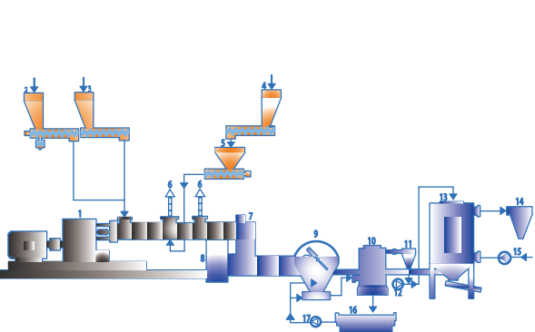
双阶偏心水雾切粒 Two Stage Eccentric Water-fog Pelletizing
