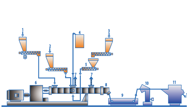
拉条切粒( 适用于增强、填充、合金、着色 ) Strand Pelletizing (suitable for reinforcement, filling, alloy and masterbatch)
