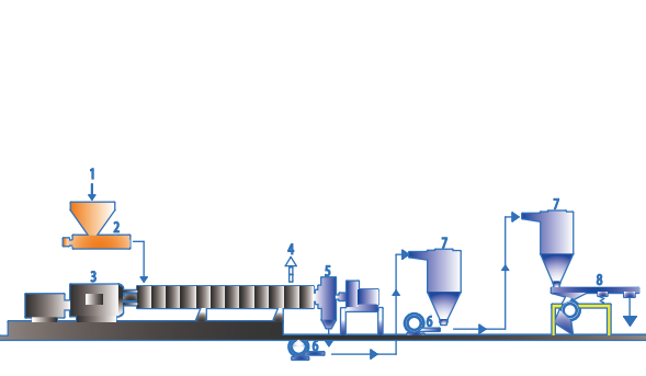
风冷造粒生产线 Air-cooling Pelletizing
